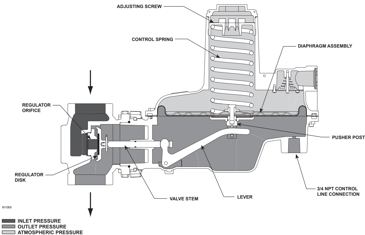
Figure 4. Type CS800EN Externally Registered Regulator Operational Schematic
