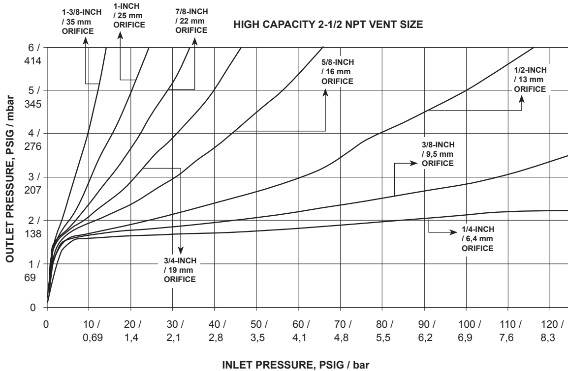
Figure 13. Types CS800IQ High Capacity Relief Curves (Blocked Open per Orifice Size) at 1 psig / 0,07 bar Set Pressure
