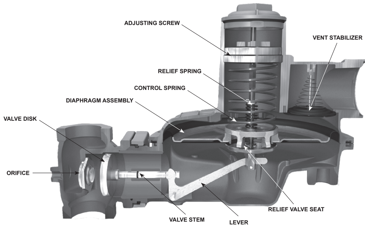
Figure 2. CS800 Series Internal View
