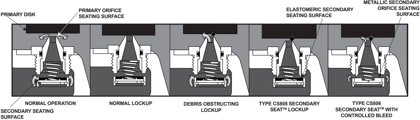
SECONDARY SEAT™ DETAILED VIEW
